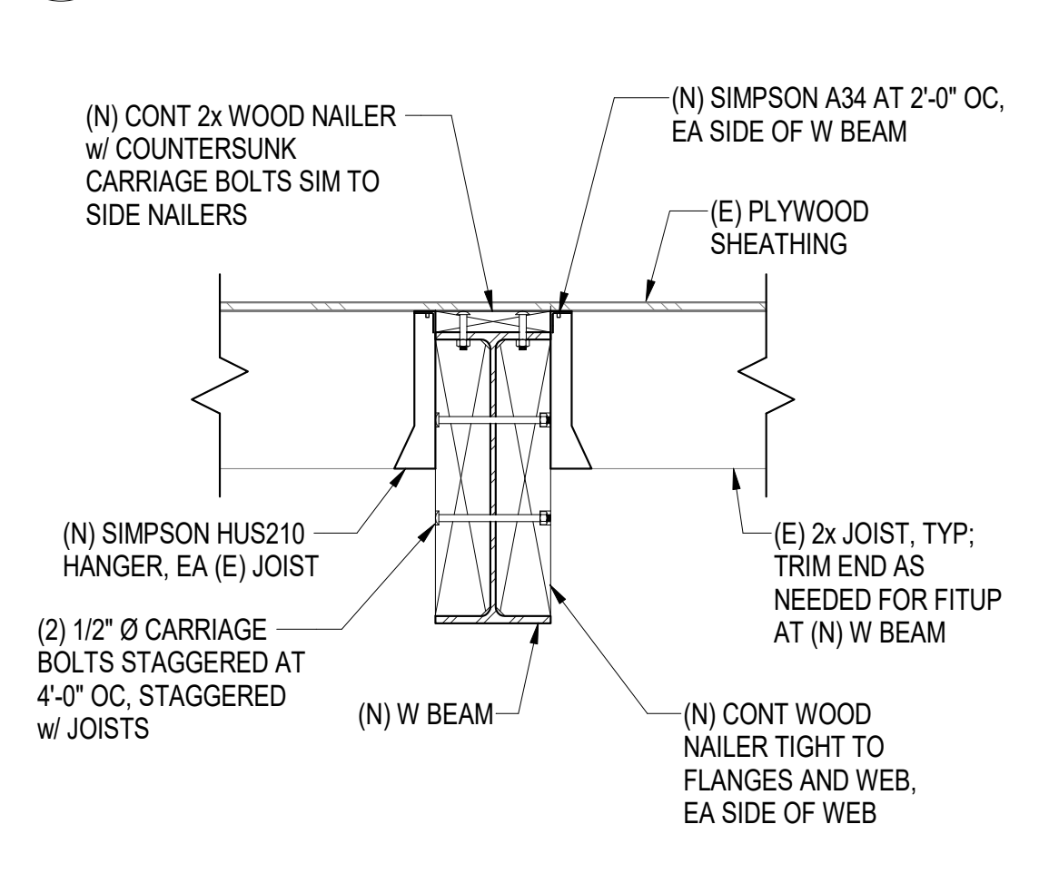
2 SECTION AT (N) W BEAM S0.1 1" = 1'-0"
