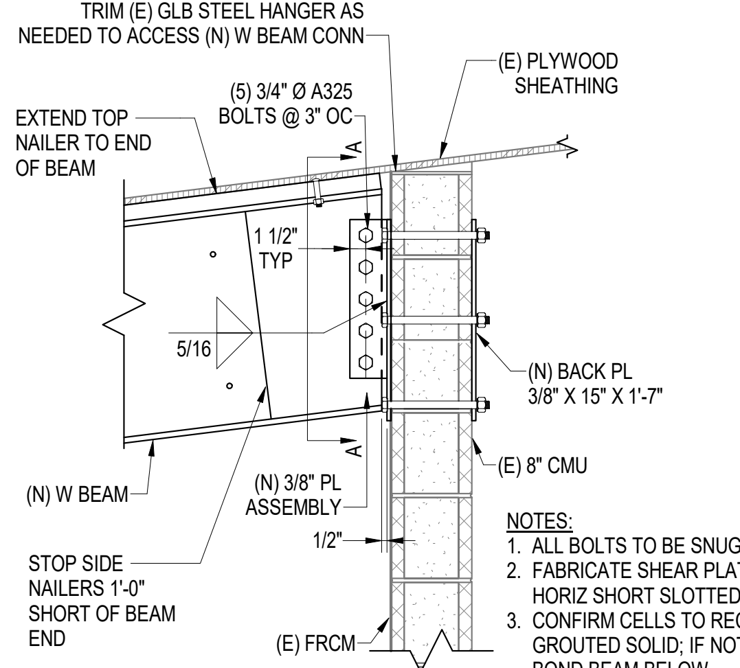
3 (N) W BEAM TO (E) CMU WALL S0.1 1" = 1'-0"
