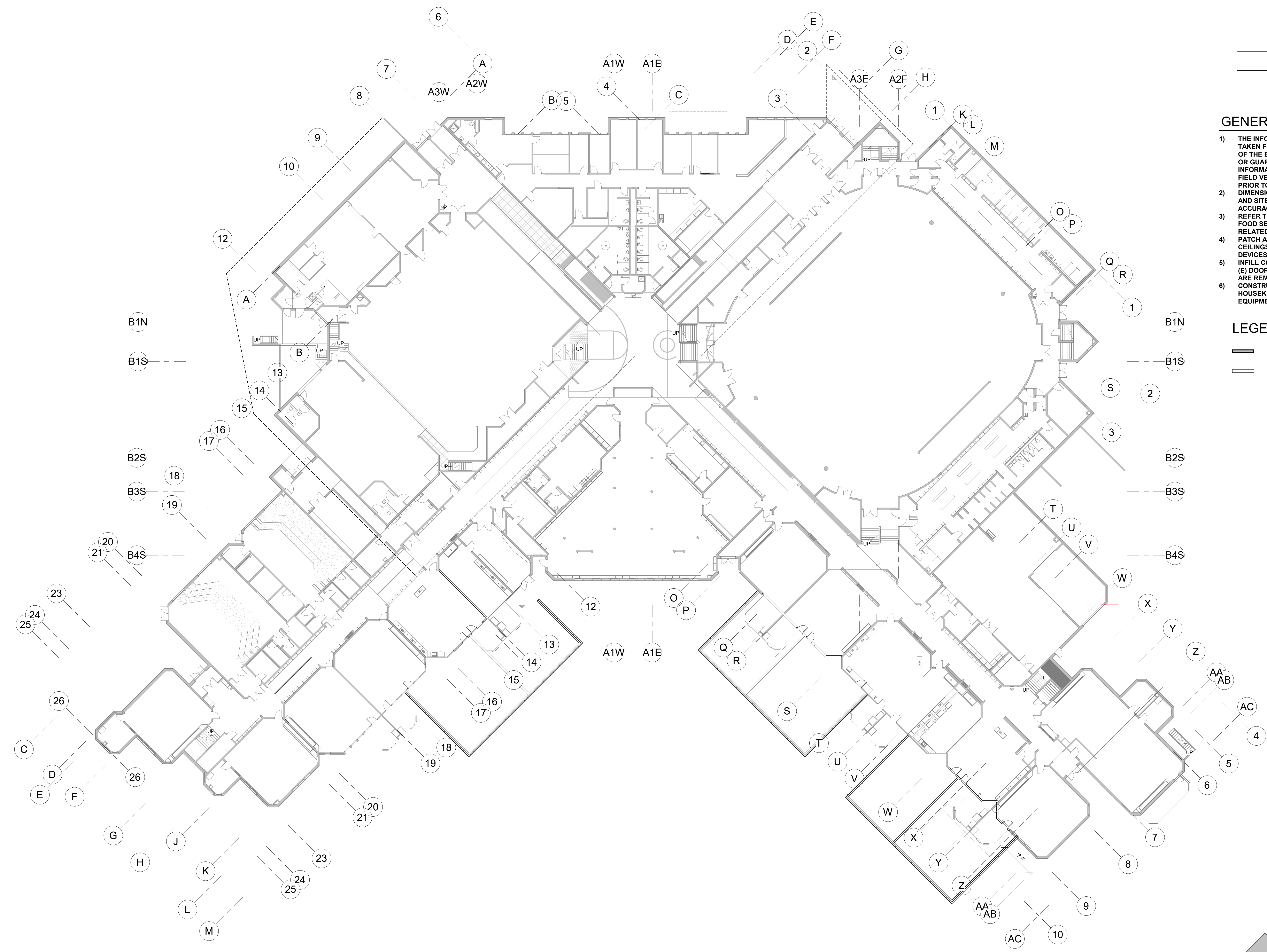
2 FLOOR PLAN - LEVEL 1 - OVERALL A210 1/16" = 1'-0"
