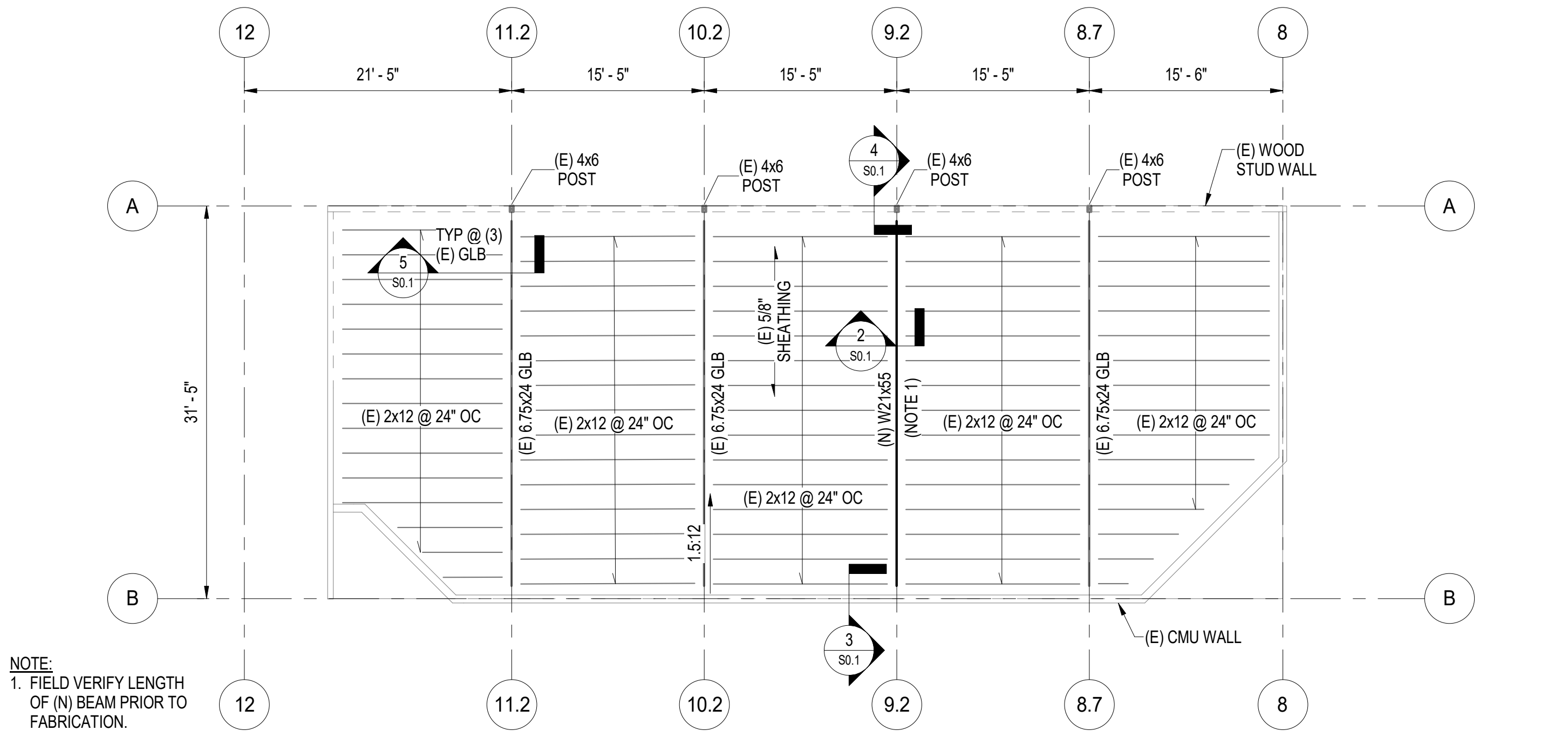
1 ROOF PLAN - BOILER ROOM S0.1 1/8" = 1'-0"
