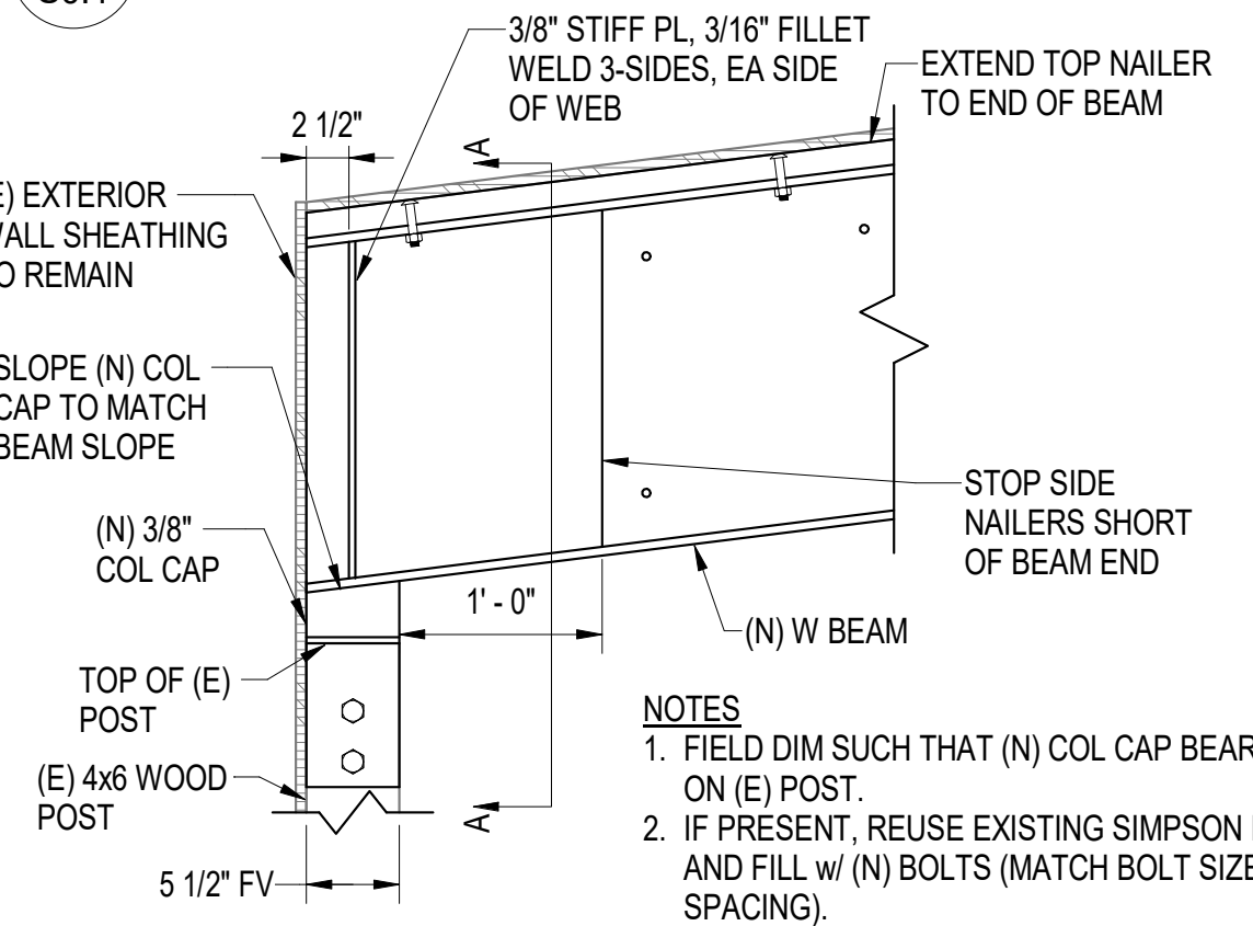
4 (N) W BEAM TO (E) WOOD POST S0.1 1" = 1'-0"
