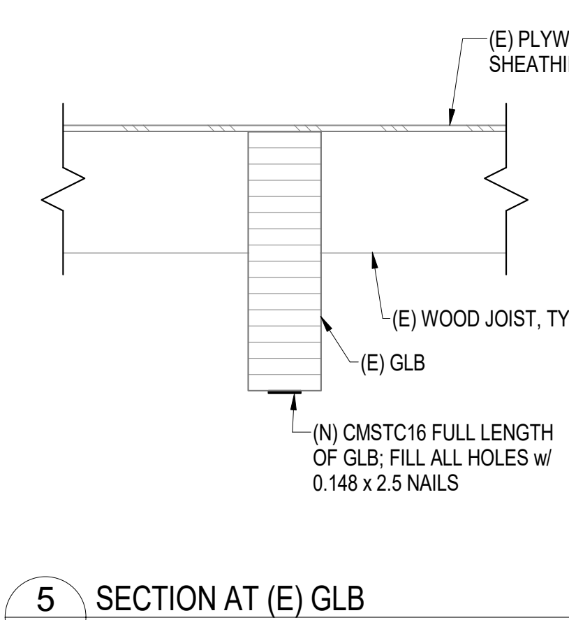
5 SECTION AT (E) GLB S0.1 1" = 1'-0"
