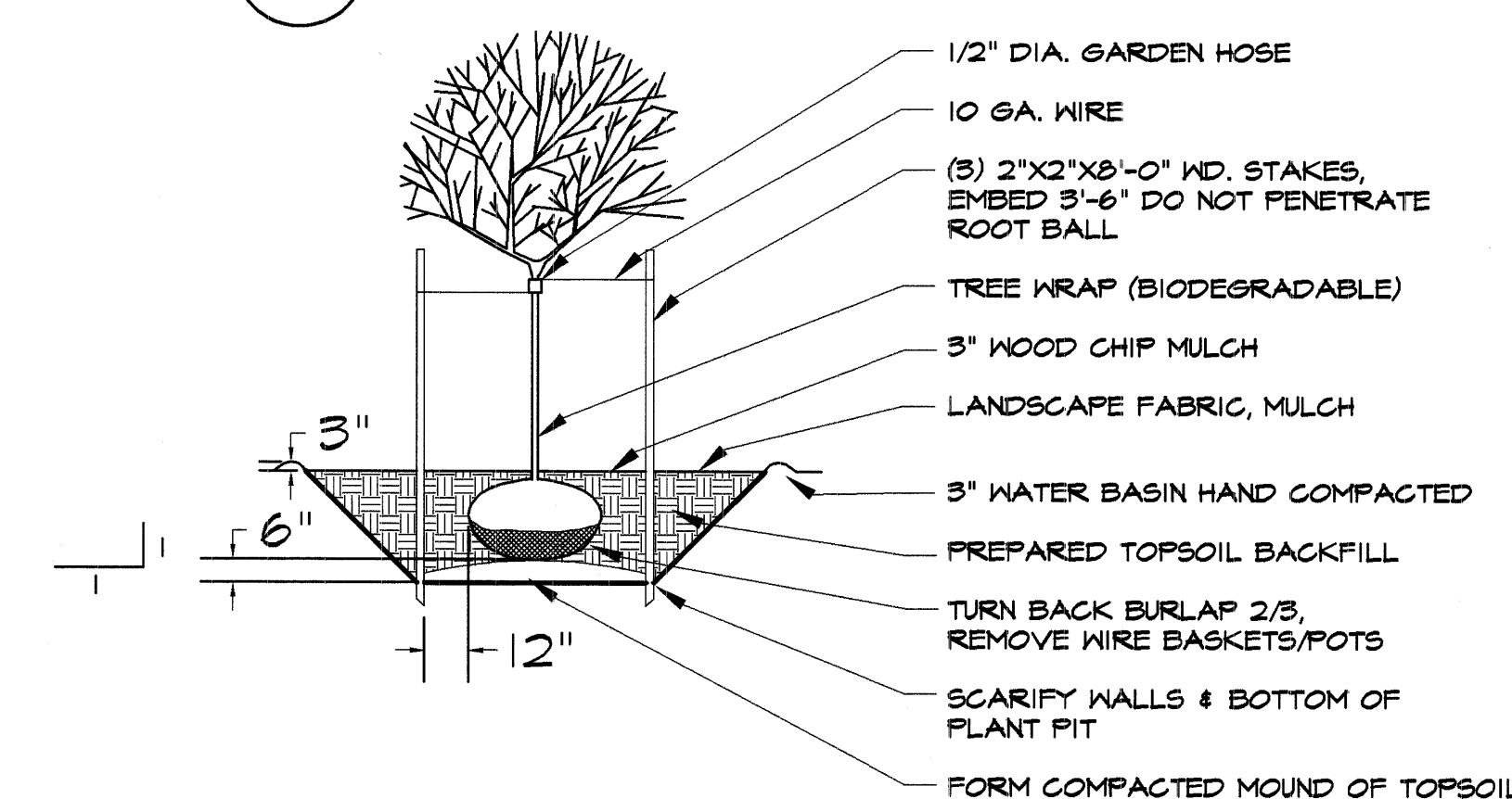
2 TYPICAL DECIDUOUS TREE PLANTING LI SCALE: NTS
