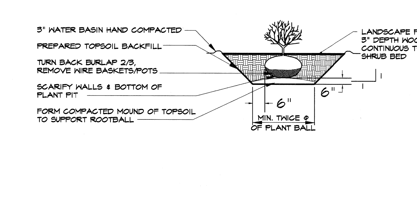
4 TYPICAL SHRUB PLANTING LI SCALE: NTS
