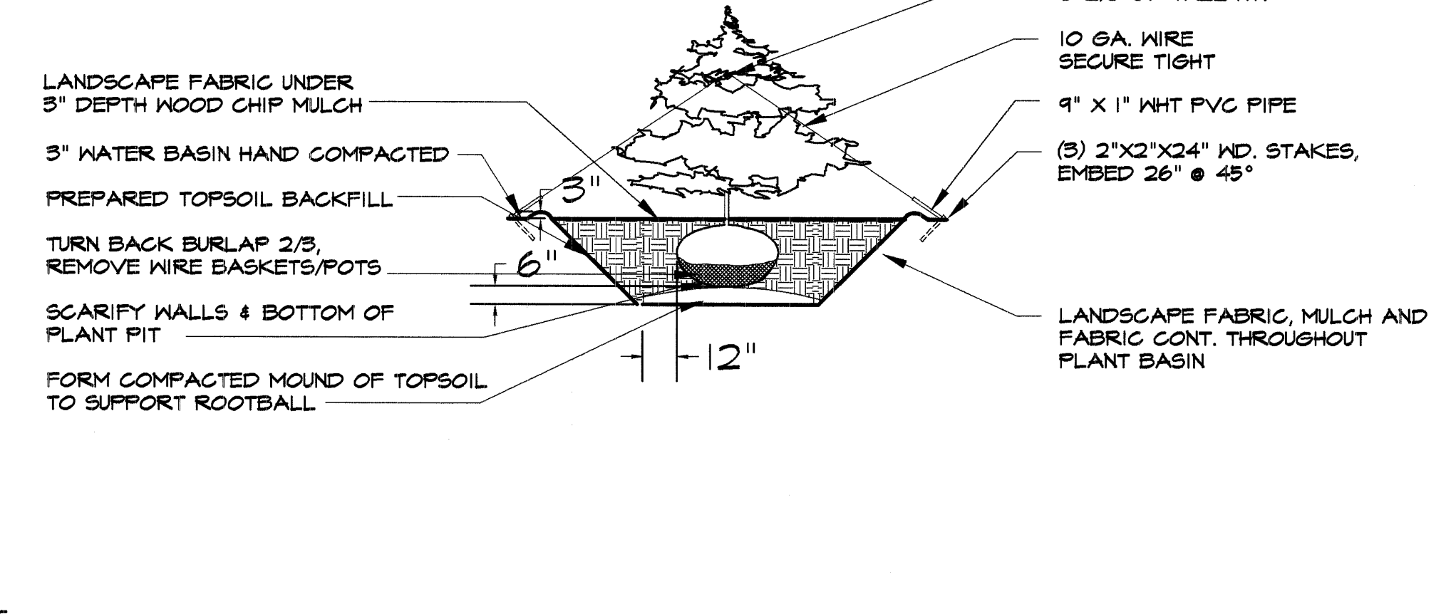
3 TYPICAL EVERGREEN TREE PLANTING LI SCALE: NTS
